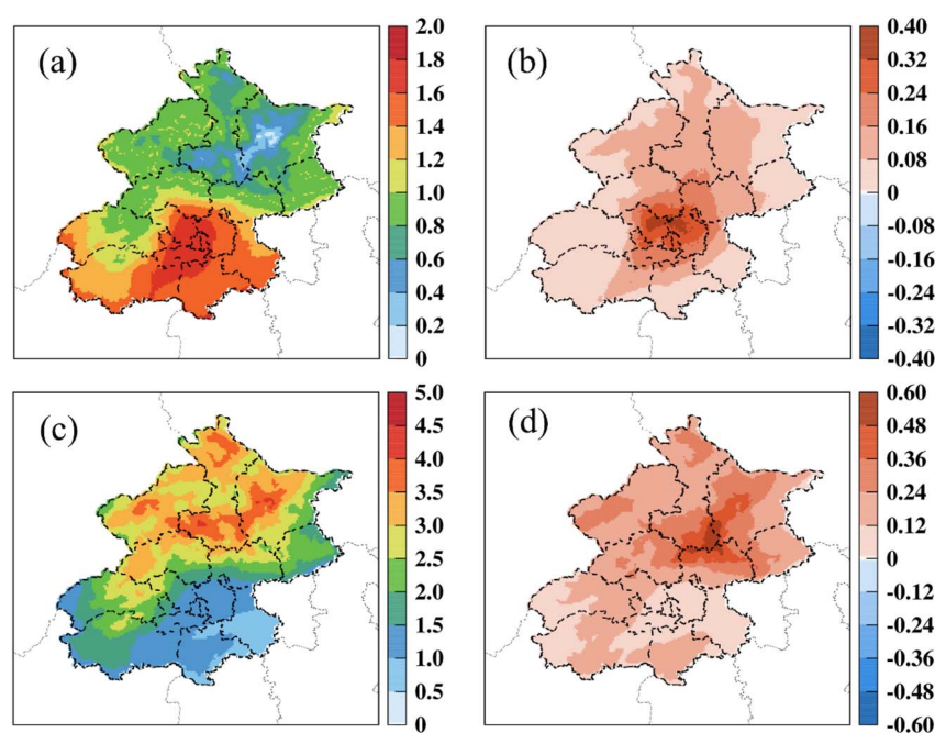
Fig. 6 (a) The contributions to SOA concentrations formed by BVOC emissions (BSOA) from urban green spaces and (b) the difference between the B5 case and the B4 case ( \text{B5} - \text{B4} ). (c) The contributions to BSOA concentrations from rural vegetation and (d) the difference between the B5 case and the B4 case; the unit is \mu\text{g m}^{-3} .
