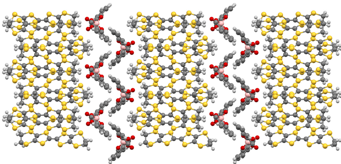
Fig. 10 Double anion layer in \kappa\text{-(BEDT-TTF)}_2[B_6/5(\text{salicylate})_2] .
