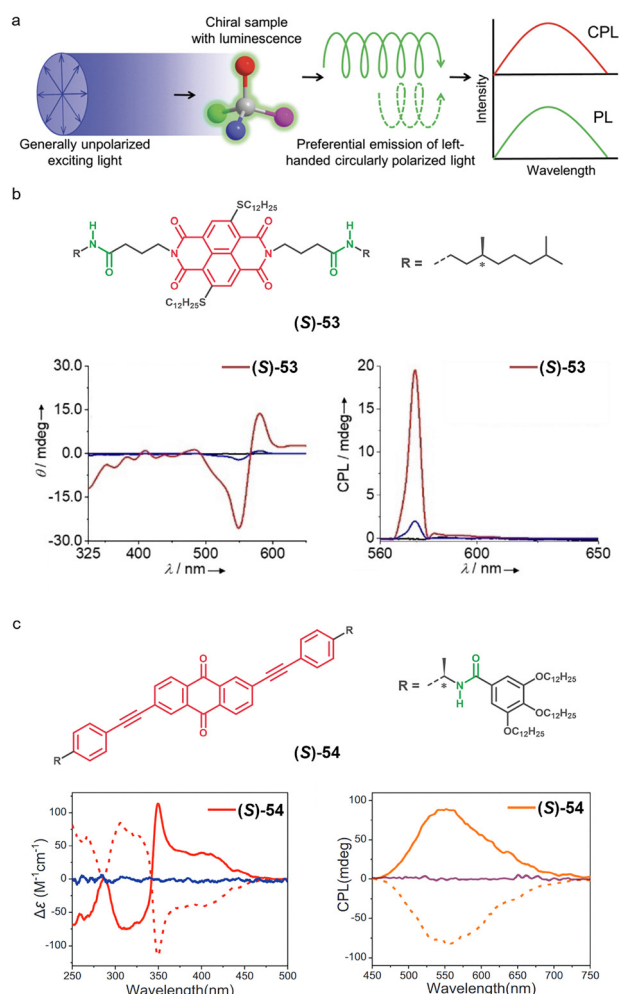
Fig. 14 (a) Schematic representation of the circularly polarized luminescence (CPL) phenomenon (reproduced from ref. 242 with permission of Wiley-VCH Verlag GmbH & Co. KGaA, Weinheim, copyright 2019). (b) Chemical structure of chiral sulfur-substituted naphthalene-diimide ( (S)-53 ) along with its CD and CPL spectra (red lines) in decane/THF (9 : 1) ( c = 0.1 mM) (reproduced from ref. 252 with permission of Wiley-VCH Verlag GmbH & Co. KGaA, Weinheim, copyright 2020). (c) Chemical structure of chiral anthraquinone derivative ( (S)-54 ) along with its CD (red line) and CPL ( \lambda_{\text{ex}} = 365 nm) (orange line) spectra in MCH ( c = 20 mM) (reproduced from ref. 239 with permission of Wiley-VCH Verlag GmbH, copyright 2025).
