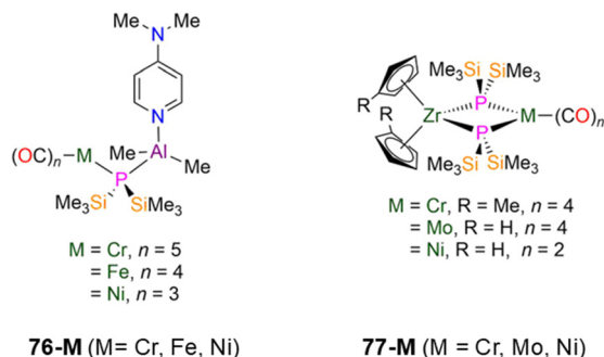
Fig. 22 Heterometallic P'' complexes [M(CO) n (μ-P'') 2 {Al(dmap)(Me) 2 }] ( 76-M ; M = Cr, n = 5, 76-Cr ; M = Fe, n = 4, 76-Fe ; M = Ni, n = 3, 76-Ni ), [Zr(Cp) 2 (μ-P'') 2 M(CO) n ] ( 77-M ; M = Mo, n = 4, 77-Mo ; M = Ni, n = 2, 77-Ni ).
