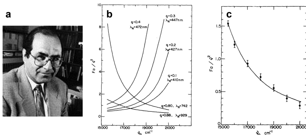
Fig. 6 (a) Photograph of Martin Moskovits. (b) The dependence of the quantity F_0/v_0^2 on exciting frequency v_0 for various values of \lambda_R , which is the resonance wavelength. The Raman intensity is proportional to F_0/v_0^2 . q is the volume fraction of the metal within a dielectric of dielectric constant \epsilon_0 . The quantity plotted is actually 6.69 \times 10^7 F_0/v_0^2 . (c) The solid line is the one of \lambda_R = 929 \text{ nm} in (b). Points are taken from ref. 72 and refer to the 1008 \text{ cm}^{-1} ring vibration of pyridine. Reproduced from ref. 4 with permission. Copyright 1978 AIP publishing.
