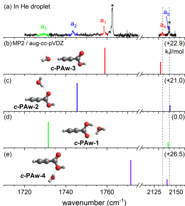
Fig. 6 Comparison of (a) the experimental IR spectrum of the c-PA \cdots \text{D}_2\text{O} 1:1 complex (peaks a_1 , a_2 , a_3 , a_4 and a_5 ) with the MP2/aug-cc-pVDZ calculated harmonic IR spectra for the lowest energy structures (b) c-PAw-3 , (c) c-PAw-2 , (d) c-PAw-1 and (e) c-PAw-4 . Structural assignments are denoted by color coding. \Delta E_0 ( \text{kJ mol}^{-1} ) are in parenthesis. Peaks belonging to the c-PA monomer in trace a are marked with asterisks. The peak position of the overlapped feature a_5 is shown by an arrow in blue. Dashed lines are used as a guide to the eye for the >2000 \text{ cm}^{-1} region.
