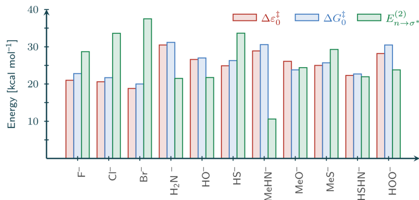
Fig. 5 Electronic ( \Delta\varepsilon_0^+ ) and Gibbs free ( \Delta G_0^+ ) intrinsic barriers and second-order hyperconjugative stabilization energies ( E_{n \rightarrow \sigma^*}^{(2)} ) for each nucleophile, computed at the MP2-SMD(THF)/cc-pVTZ level.
