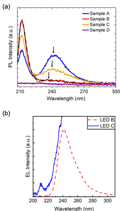
Fig. 9 (a) RTPL of different bulk AlGa 0.2 N nanowire samples ( i.e. , without any quantum wells or quantum disks) using different Al sources. Samples A, B, C, and D are the same samples as shown in Fig. 8 for SEM studies. The black dot/dash curves are deconvoluted PL peaks. The details on the PL experiments can be found in ref. 89. (b) RT EL of AlGa 0.2 N nanowire LEDs, correlating to the schematic shown in Fig. 7, using the two different Al sources. The measurement details can be found in ref. 85. The LED identification ( i.e. , LED B, LED C) from the original study is used. There are no correlations between LED B and sample B and between LED C and sample C.
