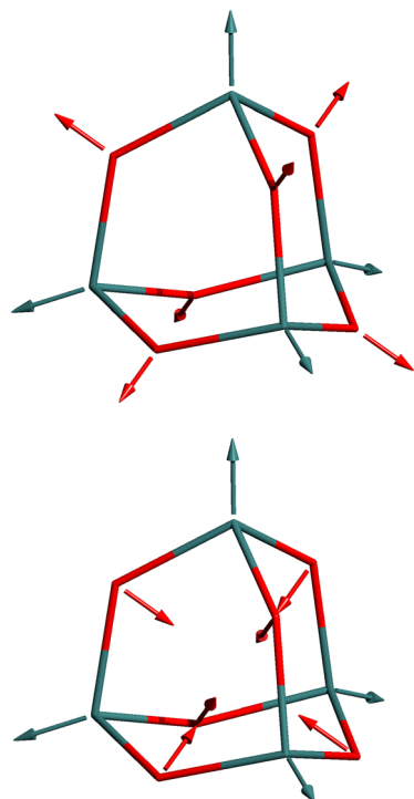
Fig. 2 The molecular structure of As 4 O 6 presented in the wireframe model and symmetry coordinates of molecular deformations: scaling \zeta (top) and distortion \eta (bottom). Arsenic and oxygen atoms denoted green and red, respectively.
