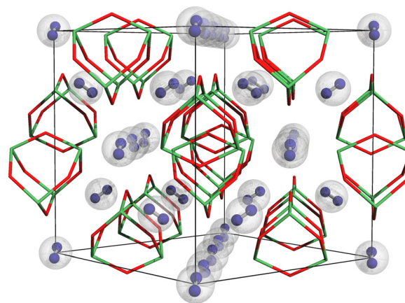
Fig. 3 Crystal structure of arsenolite inclusion compounds with helium and hydrogen, As 4 O 6 ·2He and As 4 O 6 ·2H 2 . As 4 O 6 molecules are presented in the wireframe model with As and O atoms denoted green and red, respectively. Helium atoms are presented as grey transparent spheres, whereas hydrogen molecules are shown in blue in the ball-and-stick model. Helium atoms and dihydrogen molecules are located at the 0, 0, 0 position. The most likely orientation of H 2 molecules along \langle 111 \rangle crystallographic direction is shown. Adapted from P. A. Gur'ka, L. Zhu, T. A. Strobel and J. Zachara, J. Chem. Phys. , 2020, 153 , 054501, 12 with the permission of AIP Publishing.
