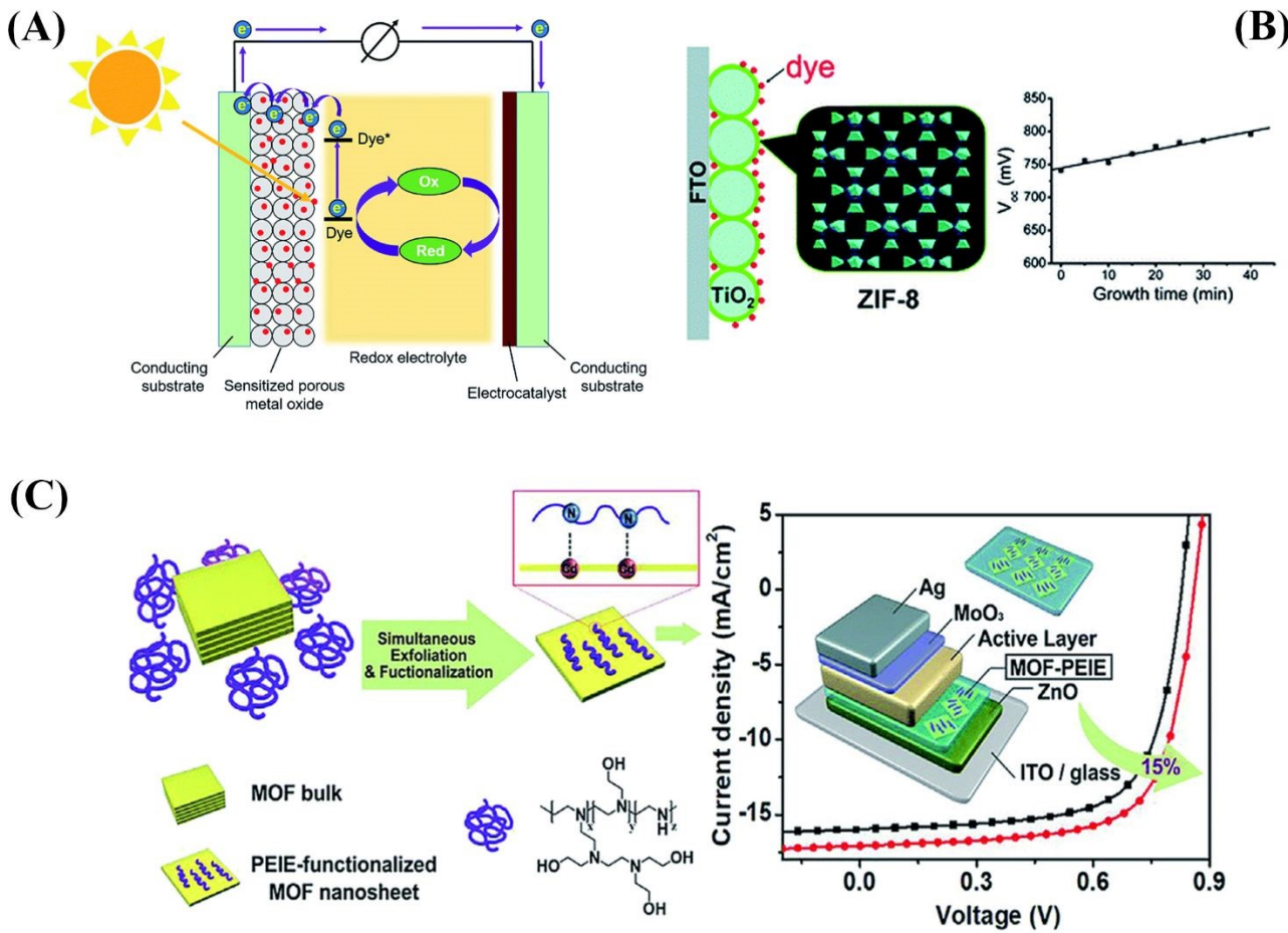
Fig. 4 (a) Schematic representation of typical dye-sensitized solar cells. (b) The use of MOFs for the photoanodes in DSSCs as the blocking layer [72]. (c) Schematic illustration of the preparation of 2D MOF nanosheets and their modified electron-extraction layer for photovoltaic devices [78].
