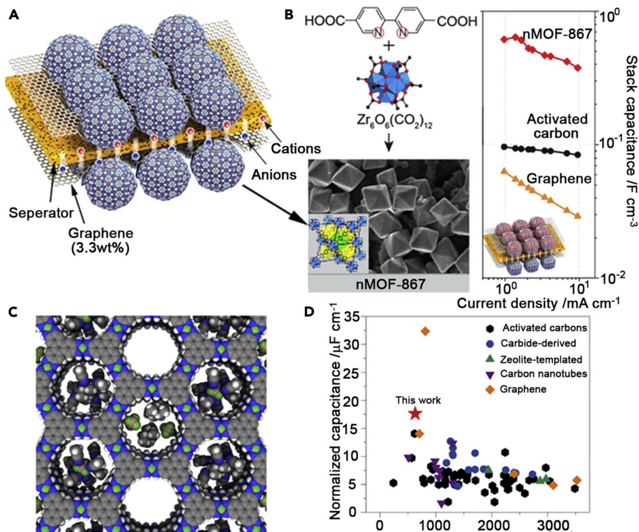
Fig. 3 MOF-Based Supercapacitors (A) Schematic construction MOF supercapacitors [54]. (B) Structure and nanocrystal morphology of nMOF-867 and comparison of stack capacitances among various EDLC materials [51]. (C) A space-filling diagram of idealized \text{Ni}_3(\text{HITP})_2 (Ni, green; F, lime; N, blue; C, gray; B, brown; H, white) [51]. (D) Comparison of BET-surface-area-normalized areal capacitances among various EDLC materials [62].
