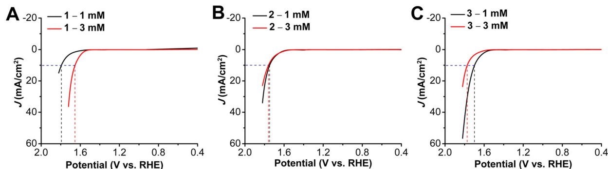
Fig. 5 LSVs for OER performance of 1 \text{ mM} and 3 \text{ mM} ink solutions of complexes (A) 1 (B) 2 and (C) 3 . Obtained with 1 \text{ cm}^2 carbon paper coated with a catalyst ink containing Vulcan carbon, Nafion, and given concentration of indicated complex as the working electrode. All experiments performed under \text{N}_2 saturation in 1.0 \text{ M KOH} ; Pt wire electrode, Hg/HgO reference electrode; 100 \text{ mV s}^{-1} scan rate.
