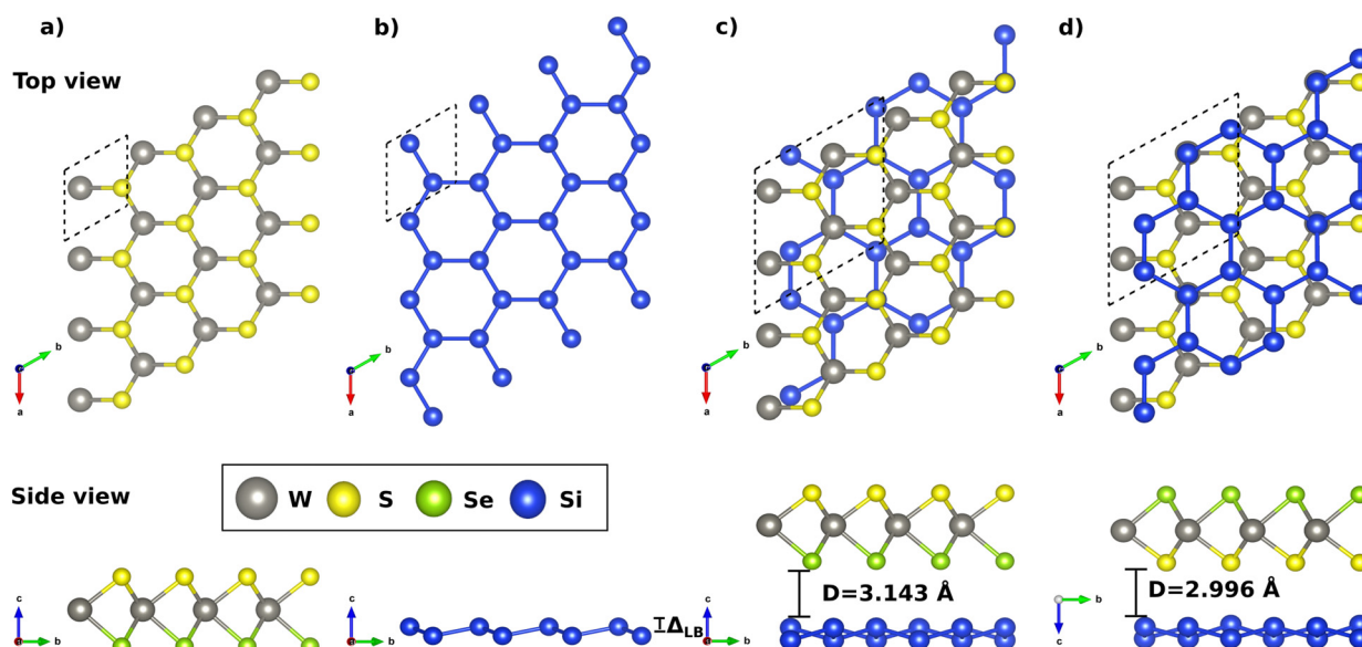
Fig. 1 The fully relaxed geometries are shown, where (a) represents the WSe Janus monolayer, (b) the silicene monolayer, and (c) and (d) the WSeS/Si (Se atoms are the shortest distance from Si atoms) and WSeS/Si (S atoms are the shortest distance from Si atoms) heterostructures, respectively.
