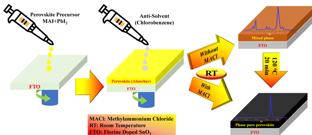
Fig. 1 Schematic representation of room temperature formation of MAPI perovskite thin-films with the addition of MACl under ambient conditions.
