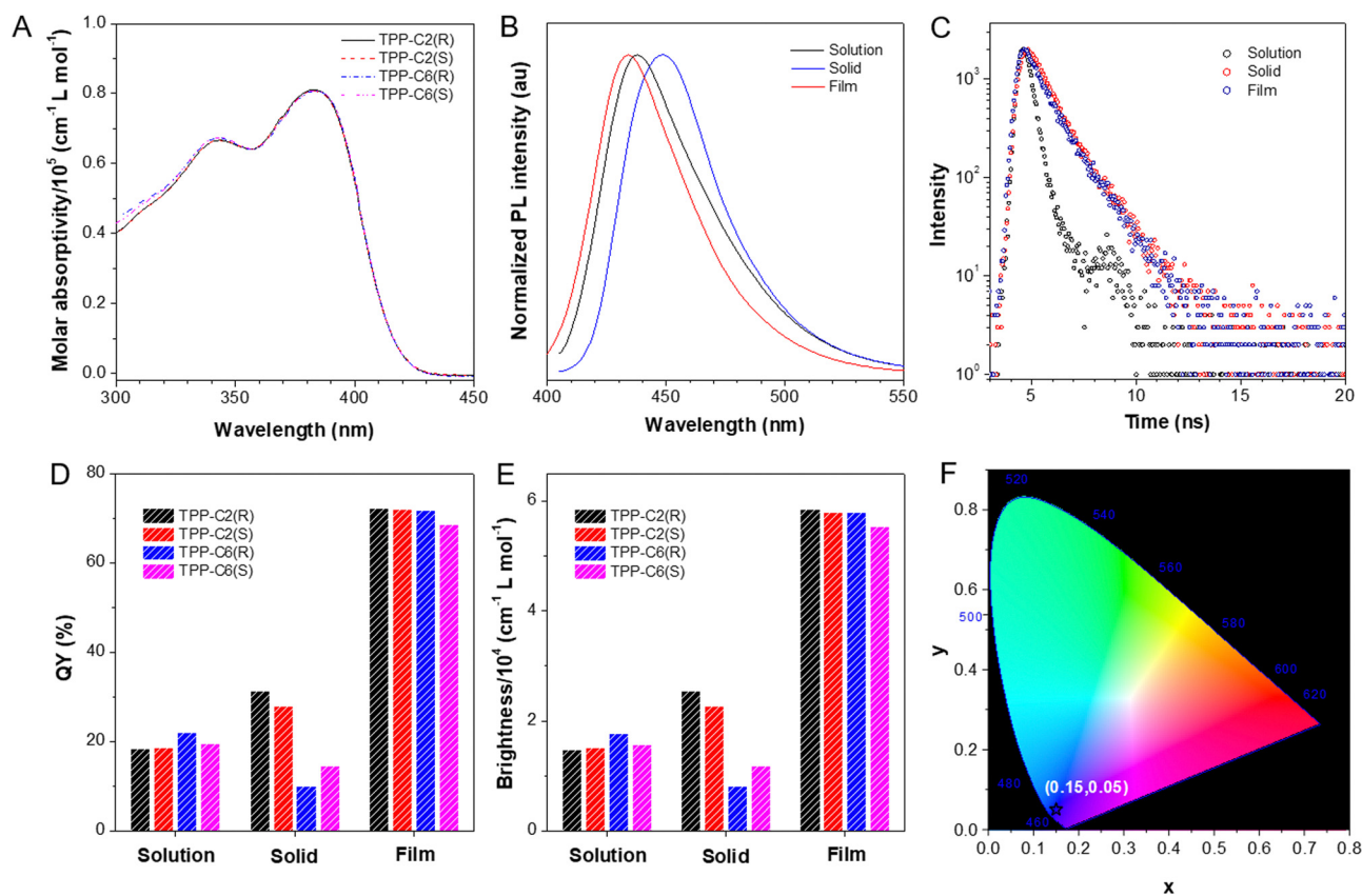
Fig. 1 (A) UV-Vis spectra of dyes in THF (10 μM). PL (B) spectra and (C) decay curves of TPP-C2(R) in solutions, powders and PMMA films. (D) Quantum yield (QY) and (E) brightness of dyes in solutions, powders and PMMA films. (F) CIE coordinate of dyes in PMMA films.
