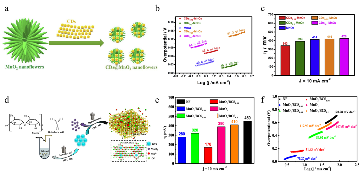
Fig. 13 The preparation method and OER performance of CDs - MnO_2 and MnO_2/BCS . (a) Synthetic illustration of CDs - MnO_2 . (b) Tafel slopes and (c) Overpotentials of different CDs - MnO_2 . Reproduced with permission. 107 Copyright 2019, Elsevier. (d) Synthetic illustration of BCS and the derived MnO_2/BCS composites. (e) Histogram of the obtained overpotentials of MnO_2/BCS_{0.04} , MnO_2/BCS_{0.06} , MnO_2/BCS_{0.08} , MnO_2/BCS_{0.1} and pristine MnO_2 . (f) Tafel plots. Reproduced with permission. 108 Copyright 2022, IOP.
