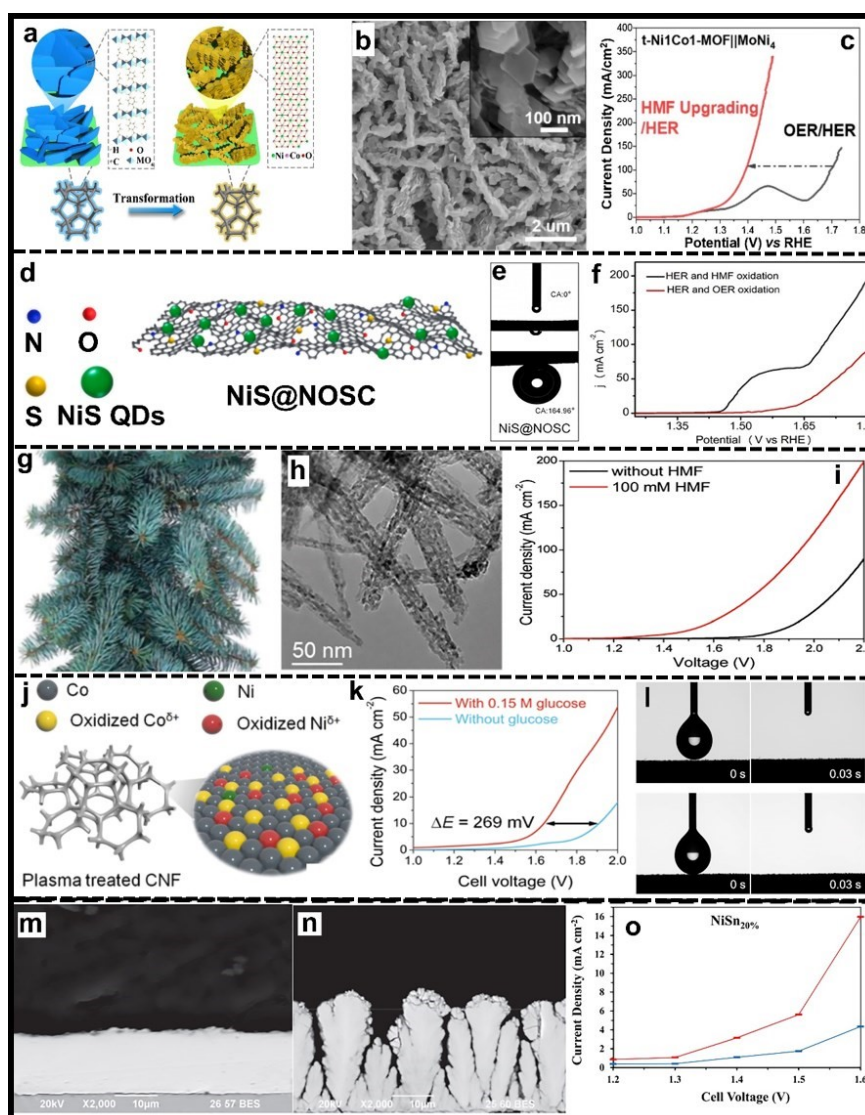
Fig. 6. Selected examples for Surface engineering subsection: (a) The illustration of nanoplaclet-on-nanoarray t-NiCo-MOF electrocatalyst deposited on NF, (b) SEM images of transformed Ni 1 Co 1 -MOF (t-Ni 1 Co 1 -MOF), and (c) LSV of t-Ni 1 Co 1 -MOF(anode) | MoNi 4 (cathode) system for OER/HER and HMFOR/HER (These figures have been reproduced from Ref. 96 with permission from Elsevier, copyright 2020), (d) Illustration of the synthesis procedure of NiS@NOSC, (e) static-water-droplet contact angles for under-water air-bubble contact angles on the surface of NiS@NOSC, (f) LSV curves of NiS@NOSC | NiS@NOSC for OER/HER and HMFOR/HER (These figures have been reproduced
