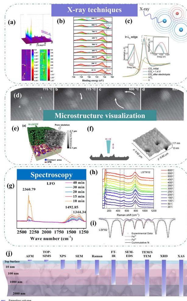
Fig. 8 (a) In situ XRD patterns of SFRuM upon switching between a reducing and oxidizing atmosphere at 800 °C and corresponding depth profile of XRD patterns. Reproduced from ref. 78. Copyright 2021, Springer Nature. (b) In situ XPS. Reproduced from ref. 115. Copyright 2020, The Royal Society of Chemistry. (c) In situ Ir L3-edge XANES spectra. Reproduced from ref. 80. Copyright 2023, Oxford University Press. (d) STEM micrographs of grains monitored in situ . Reproduced from ref. 112. Copyright 2023, Springer Nature Limited. (e) 3D reconstructed architecture image. Reproduced from ref. 93. Copyright 2024, Springer Nature. (f) AFM image. Reproduced from ref. 73. Copyright 2015, Springer Nature Limited. (g) Quasi in situ IR absorbance spectra. Reproduced from ref. 122. Copyright 2021, Elsevier. (h) In situ high-temperature Raman spectra. Reproduced from ref. 123. Copyright 2023, Elsevier. (i) Mössbauer spectra. Reproduced from ref. 114. Copyright 2021, Elsevier. (j) Schematic of typical analysis depths for techniques.
