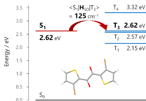
Fig. 4 Energy diagram of 1a in the S_1 -optimized trans -planar (TP) geometry. Energies and the spin-orbit coupling matrix element between the S_1 and T_3 states ( \langle S_1 | \hat{H}_{SO} | T_3 \rangle ) were calculated at the TDA/uCAM-B3LYP-D3/6-311G(d) level of theory.
