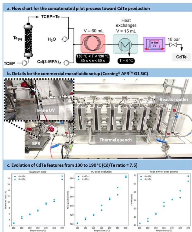
Fig. 12 (a) Simplified flow chart of the mesofluidic setup used for the scalability trials toward \text{CdTe} (b) photograph of the experimental setup, featuring a Corning® Advanced-Flow Reactor™ G1 SiC (60 mL of internal volume). (c) Comparison of the \text{CdTe} QDs main characteristics (prepared at temperatures ranging from 130 °C to 190 °C and residence times of 45 s or 60 s).
