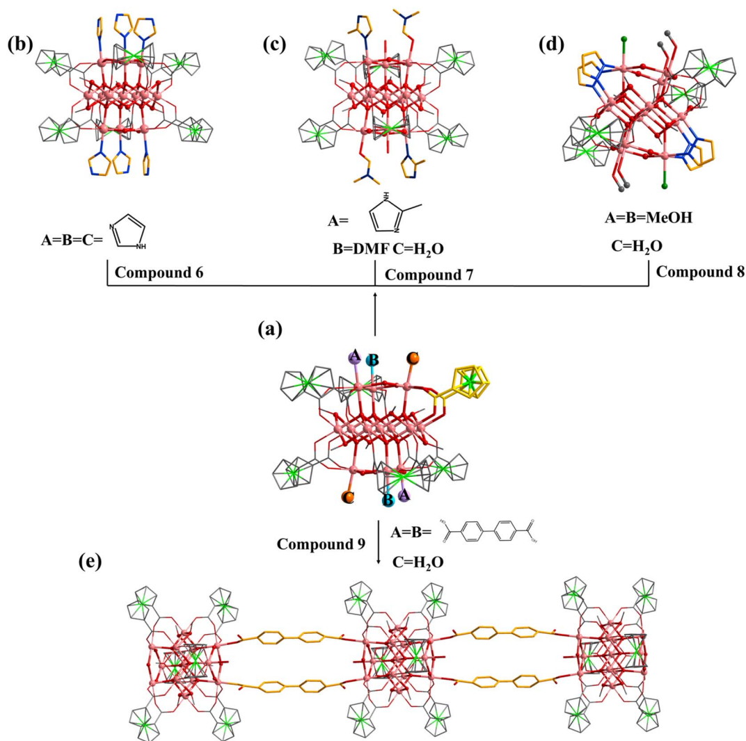
Fig. 5 (a) [In_{13}] as a secondary building unit; (b) compound 6 (A = B = C = HIm); (c) compound 7 (A = 2-mim, B = DMF, C = \equiv H_2O ); (d) compound 8 (A = B = MeOH, C = \equiv H_2O ); (e) compound 9 (A = B = BPDC, C = \equiv H_2O ). A, B and C represent different substitution sites.
