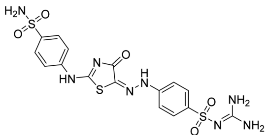
N-(Diaminomethylene)-4-(2-(4-oxo-2-((4-sulfamoylphenyl)amino)thiazol-5(4H)-ylidene)hydrazinyl)benzenesulfonamide
