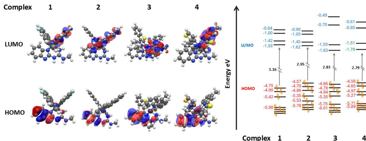
Fig. 5 (left) TD-DFT predicted HOMO and LUMO orbital distributions of complex 1–4 and (right) visualization of the energy levels of frontier orbitals with computationally obtained HOMO–LUMO gap.
