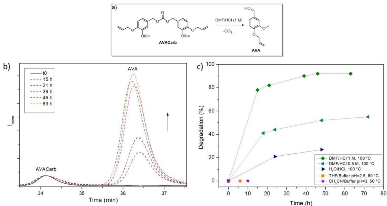
Fig. 6 (a) Molecular model: cleavage of AVACarb into AVA under acidic conditions, (b) monitoring of the degradation in DMF/HCl 1 M at 100 °C via SEC, (c) establishment of degradation conditions for AVACarb : test of different reaction conditions.
