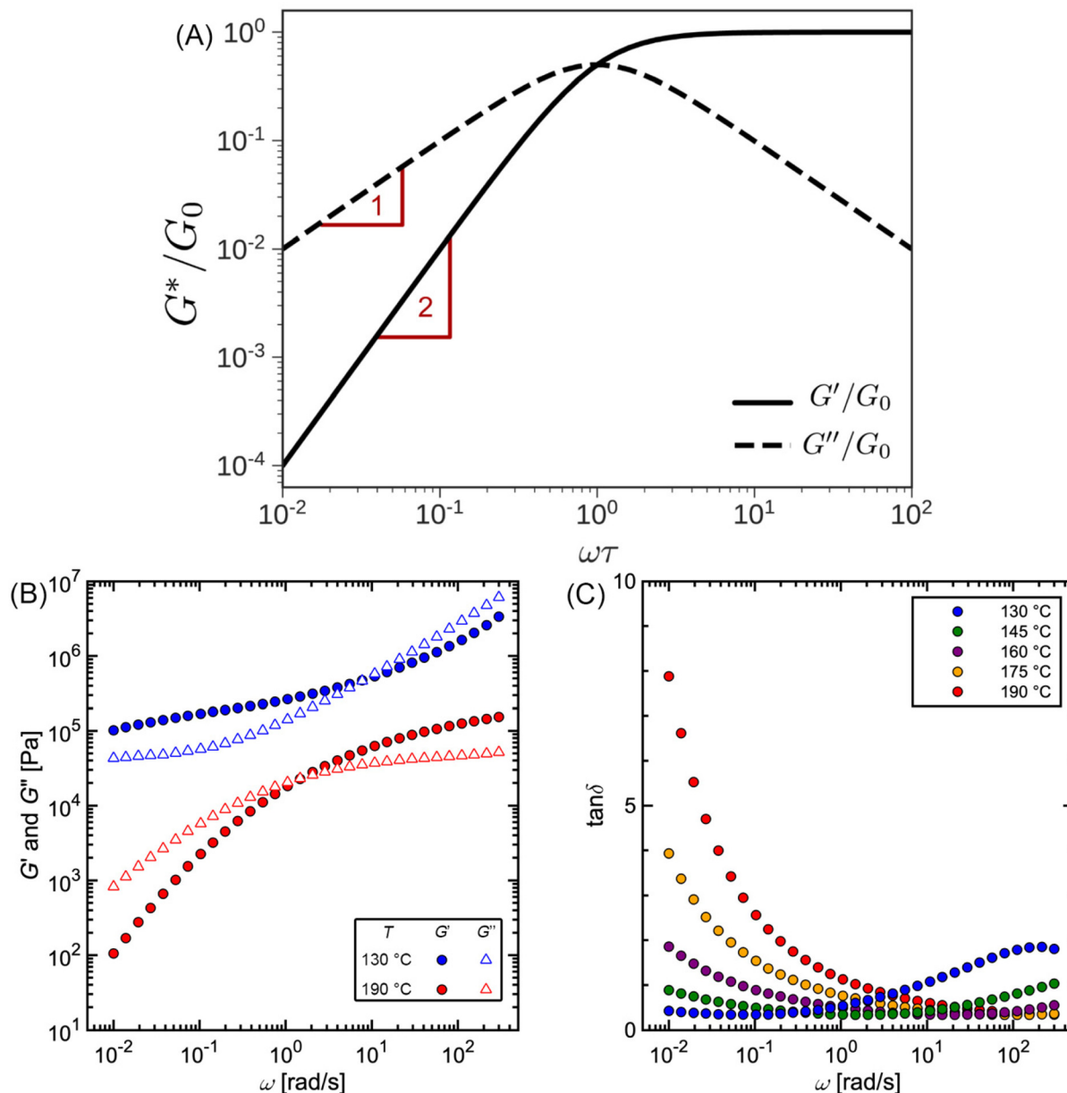
Fig. 10 (A) SAOS moduli for single mode Maxwell model. (B) SAOS moduli and (C) \tan \delta for commercial polystyrene.
