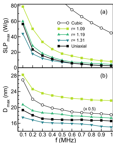
Fig. 8 Frequency dependence of the (a) maximum SLP and (b) corresponding particle size extracted from the curves in Fig. 7 for different nanoparticle elongation ratios r = 1.09, 1.19, 1.31 (colored symbols) and also for the cases of only uniaxial or only (black squares) cubic contribution (empty circles) with K_{u,c} = 1.1 \times 10^4 J/m 3 . Notice that D_{\max} for the last case has been rescaled by 0.5.
