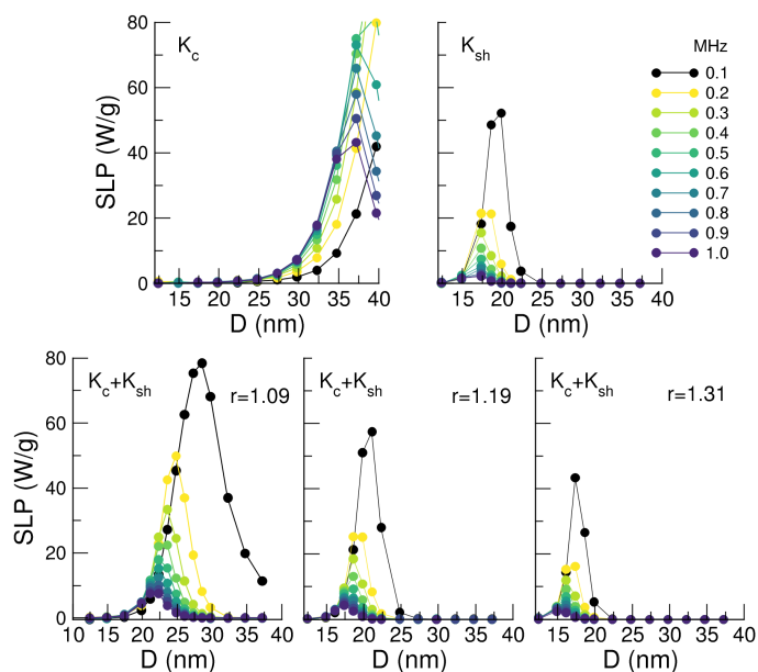
Fig. 7 Size-dependence of the SLP for different frequencies and maximum AC fields accomplishing the Brezovich criterion H_{max} \cdot f = 4.85 \times 10^8 A/m.s. Upper panels show the case for spherical particles with only crystalline cubic (left, K_c ) and only shape (right, with K_{sh} = K_c ) anisotropies, respectively. Lower panels correspond to ellipsoidal particles of aspect ratios r = 1.09, 1.19, 1.31 with uniaxial shape anisotropy added to the cubic one.
