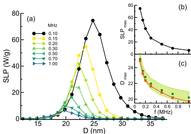
Fig. 6 (a) Dependence of the SLP on nanoparticle diameter D and aspect ratio r = 1.12 ( K_{sh} \approx 6.5 kJ/m 3 ) for the frequencies indicated in the legend, and AC fields respecting the Brezovich criterion. A cubic anisotropy constant equal to that of magnetite has been considered. (b) and (c) display the frequency dependence of the maximum value of SLP and the diameter at which is obtained, D_{max} . In (c), the green circles are the D_{max} values obtained from Eq. 3 using a value of f_0 = 10^9 Hz and the green shaded region the range obtained when varying f_0 between 0.5 - 1.5 \times 10^9 Hz.
