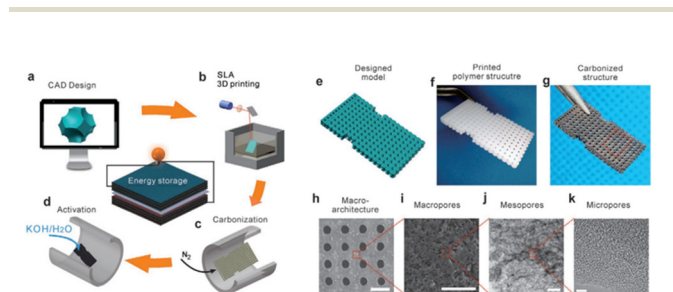
Fig. 9 Schematic of the SLA print process and SEM/TEM imaging of macroarchitectures, macropores, mesopores, and micropores with scale bars of 1 mm, 20 \mu\text{m} , 100 nm, and 5 nm, respectively. 80
