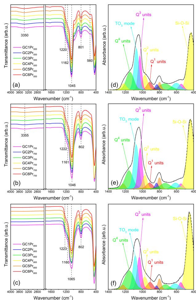
Fig. 1 ATR-IR spectra recorded for individual sol-gel materials heat-treated at 500 °C (a), 700 °C (b), and 900 °C (c). The deconvolution of spectra for representative \text{GC2Pr}_{500} , \text{GC2Pr}_{700} , and \text{GC2Pr}_{900} nano-glass-ceramics in the range from 1400 \text{cm}^{-1} to 400 \text{cm}^{-1} region is also presented in (d)–(f), respectively.
