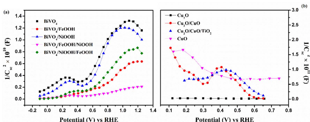
Fig. 7 Mott–Schottky plots of (a) BiVO 4 , BiVO 4 /FeOOH, BiVO 4 /NiOOH, BiVO 4 /FeOOH/NiOOH and BiVO 4 /NiOOH/FeOOH photoanodes and (b) Cu 2 O, Cu 2 O/CuO, Cu 2 O/CuO/TiO 2 and CuO photocathodes tested in 0.1 M Na 2 SO 4 (pH 6) at 1 kHz under dark conditions.
