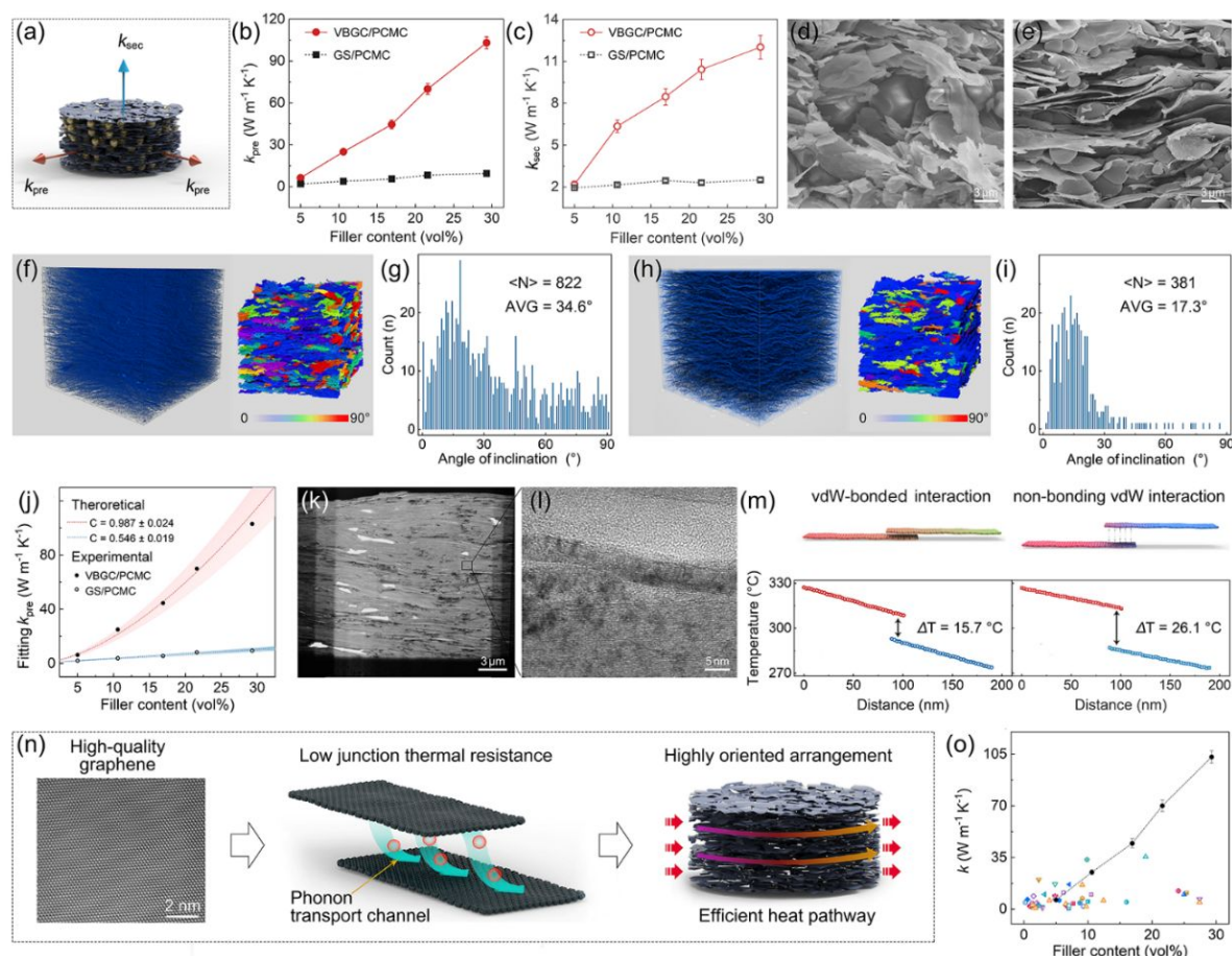
Fig. 3 (a) Schematic illustrating the thermal conductivity direction ( \kappa_{pre} and \kappa_{sec} ) of VBGC/PCMCs. The comparison of (b) \kappa_{pre} and (c) \kappa_{sec} between VBGC/PCMCs and GS/PCMCs. Cross-sectional SEM image of (d) GS/PCMCs and (e) VBGC/PCMCs. 3D XCT scanning and angle statistics of the filler for the case of (f, g) GS/PCMCs and (h, i) VBGC/PCMCs. (j) Fitting of the experimental \kappa_{pre} of VBGC/PCMCs and GS/PCMCs based on the Agari model. (k, l) TEM images illustrating vdW-bonded interfaces of adjacent graphene sheets within VBGC/PCMCs. (m) The calculated temperature distribution of adjacent graphene sheets with vdW-bonded interface and the interface formed based on the non-bonding vdW interaction through the NEMD simulation. (n) Scheme illustrating the heat-transfer mechanism of the VBGC/PCMCs. (o)
