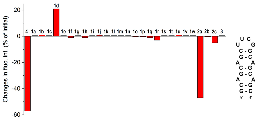
Fig. 1 Changes in the fluorescence intensity (in % of the initial intensity) of aurones 1a–1w and 2a–2c , aza-aurone 3 and furamidine ( 4 ) ( c_{\text{lig}} = 5 \mu\text{M} ) in the presence of 1 equiv. of the 5'-GCAGCAGCUUCGGCAGCAGC-3' oligonucleotide in a buffer (pH = 7); positive values indicate fluorescence light-up in the presence of RNA and negative values indicate fluorescence quenching in the presence of RNA. The fluorescence output of each ligand was measured at three different excitation wavelengths: \lambda_{\text{ex}} = 350, 400 and 450 nm. The most reliable fluorescence output was obtained upon excitation at \lambda_{\text{ex}} = 350 nm for most compounds except for 1d ( \lambda_{\text{ex}} = 450 nm) and 2b ( \lambda_{\text{ex}} = 400 nm). To ensure the reproducibility, each measurement was repeated at least three times, and the repeat experiments gave values within 20%.
