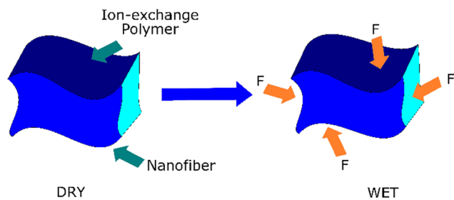
Fig. 8 Mechanism of the nanofiber suppressing the swelling of the matrix. 92,93
