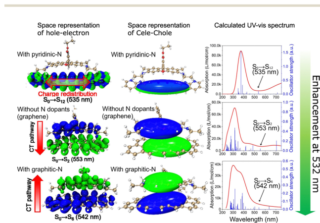
Fig. 5 Theoretical verifications for the chemical enhancement observed on the PAN-based SERS substrates. Electron–hole distribution (left), cele-chole distribution (middle), and calculated UV-vis spectra (right) of the complexes between R6G and conjugated systems with pyridinic-N dopants, without N dopants, and with a graphitic-N dopant from the ground state to the excited state during the electron excitation process obtained by time-dependent density functional theory (TDDFT) calculation with Gaussian16.
