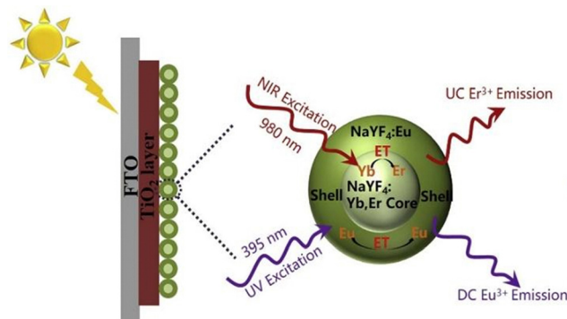
Fig. 8 Near-infrared and ultraviolet sunlight harvesting, and spectral conversion into the visible range to activate the N719 dye for the enhancement of a DSSC device. Reprinted with permission from Elsevier. 87
