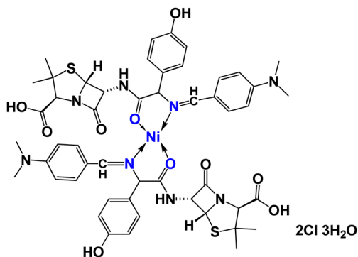
Fig. 1 Structure of [\text{Ni(II)(SB)}_2]2\text{Cl} \cdot 3\text{H}_2\text{O} .
