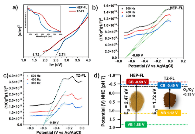
Fig. 2 (a) Tauc plot (inset DR UV-vis spectrum), Mott-Schottky plot of (b) HEP-FL and (c) TZ-FL, and (d) band energy diagram.
