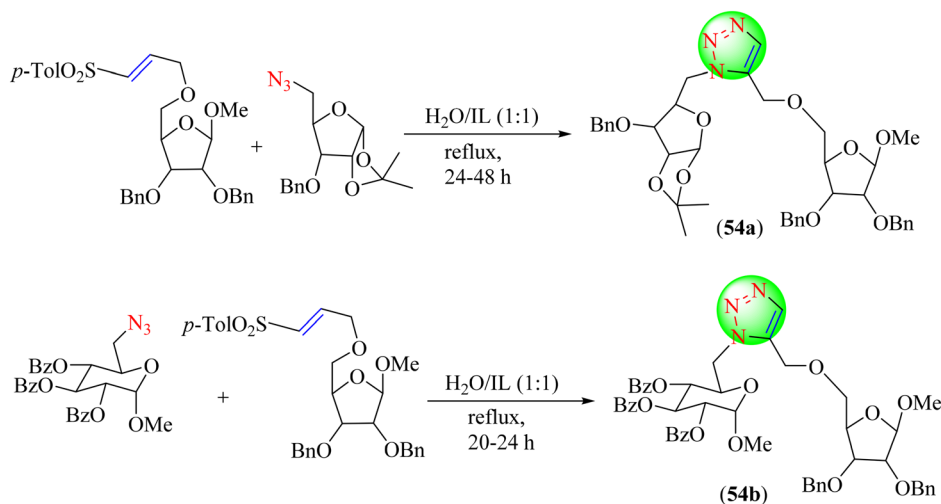
Scheme 58 Synthesis of 1,2,3-triazoles ( 54a–54b ) using ILs as the reaction media.
