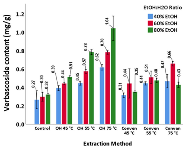
Fig. 5 Effect of extraction methods on the recovery of verbascoside from olive leaves ( \text{mg} per g leaf extract). Extraction methods: ohmic heating (OH), conventional heating (convent), and solvent extraction without heating (control). The results are presented as mean values with standard deviation error bars.
