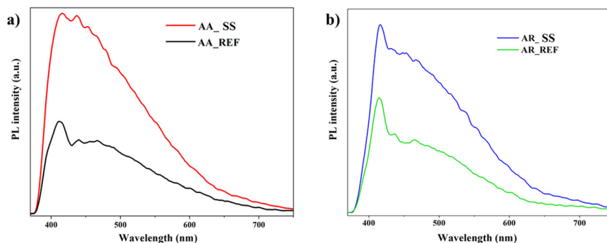
Fig. 7 Photoluminescence spectra of \text{TiO}_2 NPs: a) AA before and after immersion of soil solution; b) AR before and after immersion of soil solution.
