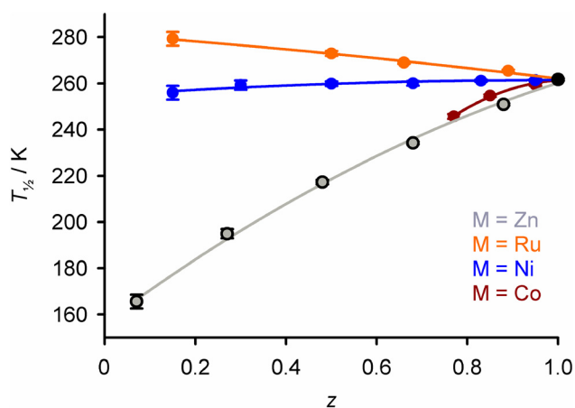
Fig. 3 Variation of T_{1/2} with composition in [\text{Fe}_z\text{M}_{1-z}(\text{1-bpp})_2][\text{BF}_4]_2 (Scheme 1) with different dopant ions. The \text{Fe}_z\text{Zn}_{1-z} data correspond to those in Fig. 2. Analogous data for other doped SCO compounds are in Fig. S1 and S2† This figure has been adapted from ref. 63 with permission from the Royal Society of Chemistry, copyright 2023.
