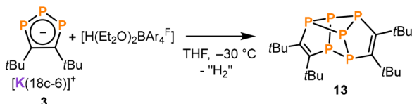
Scheme 3 Synthesis of 13 .
