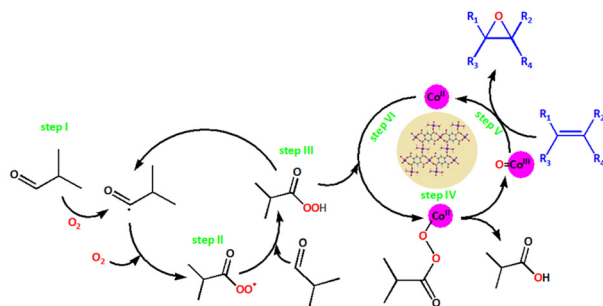
Fig. 9 Possible reaction mechanism steps for the formation of peroxy species catalysed by the heterogeneous catalyst 2 in the epoxidation of olefins. \{\text{Co}(\text{OH}_2)_2\text{O}_4\} active species is represented by \text{Co}^{\text{II}} .
