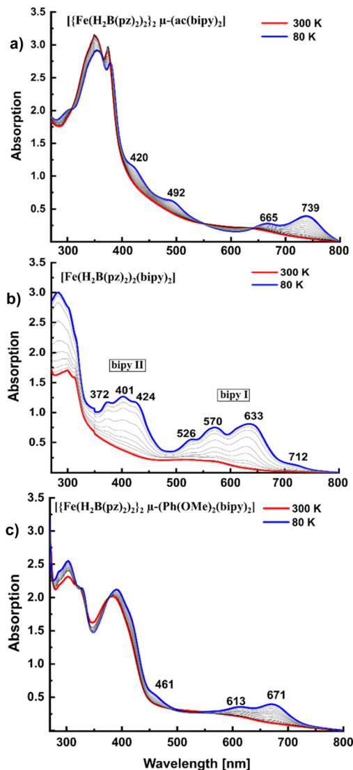
Fig. 4 Temperature dependent UV/Vis spectra of 1 crimped in KBr (a) and 2 in a polymer composite (polystyrene), (c) in comparison with the mononuclear parent compound [Fe(H 2 B(pz) 2 ) 2 (bipy)] (evaporated film on quartz glass) (b). The 300 K spectra are plotted in red, the 80 K spectra in blue and temperatures in between as grey lines. For [Fe(H 2 B(pz) 2 ) 2 (bipy)] (b) the “bipy I” and “bipy II” bands are indicated. The 712 nm band is assigned to a 3 MLCT transition (see text).
