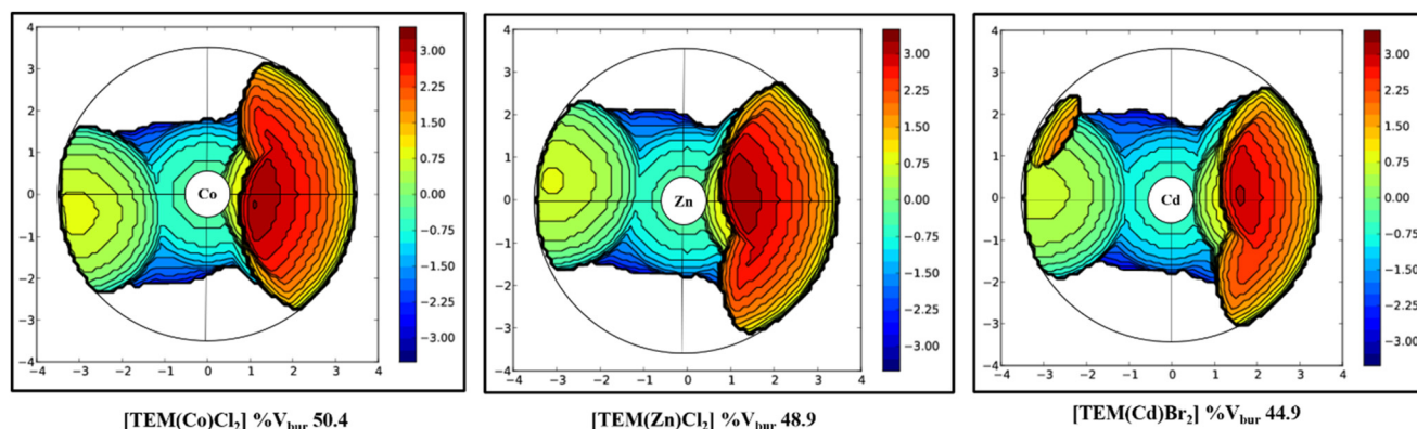
Fig. 5 Comparison of the topographic maps of [\text{TEM}(\text{M})\text{X}_2] ( \text{M} = \text{Co} and \text{Zn} ; \text{X} = \text{Cl} ; \text{M} = \text{Cd} , \text{X} = \text{Br} ), complexes.
