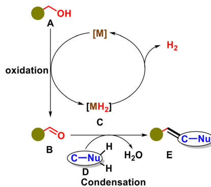
Fig. 3 General procedure for olefination via acceptorless dehydrogenative coupling.
