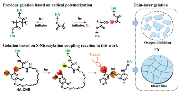
Fig. 6 Schematic depicting the photo-responsive behaviour of cyclic o -nitrobenzyl-modified hyaluronic acid (CNB-HA) in the context of periodontitis treatment. Upon irradiation with 395 nm light, CNB-HA undergoes a photochemical reaction that simultaneously generates three distinct reactive groups: thiol, nitroso, and aldehyde. Through rapid non-radical cross-linking via S -nitrosylation, the generated thiols and nitroso groups form a thin gel within 5 s. Concurrently, the aldehyde selectively binds the amino groups of the tissue, facilitating in situ adhesion and establishing a sealed environment that prevents bacterial infiltration into the wound site. Reproduced from ref. 121 with permission from Wiley. Copyright (2021).
