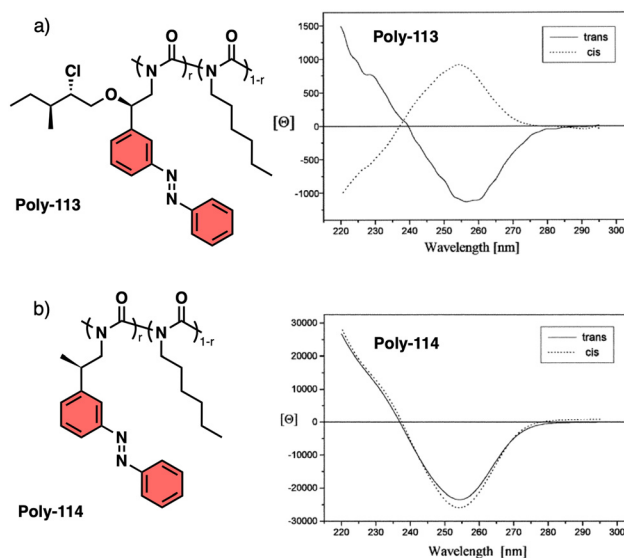
Fig. 53 Structures of PICs (a) poly- 113 and (b) poly- 114 copolymers and CD monitoring of the helical variations in the E/Z photoisomerization processes. Reproduced from ref. 276 with permission from the American Chemical Society, copyright 1998.
