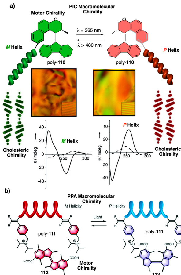
Fig. 52 (a) Helix inversion process of poly- 110 bearing a chiral photo-active molecular motor and subsequent hierarchical chiral transmission from molecular motor to helical PIC cholesteric phase. Reproduced from ref. 271 with permission from the American Chemical Society, copyright 2008. (b) Helix inversion process of PPA poly- 111 via salt-bridge formation with chiral molecular motor 112 . Reproduced from ref. 272 with permission from the Royal Society of Chemistry, copyright 2017.
