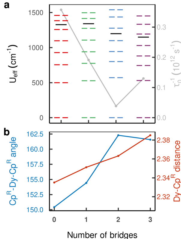
Fig. 5 (a) U_{\text{eff}} (left axis) and \tau_0^{-1} (right axis) Arrhenius parameters of the over-barrier Orbach process. The values of the anisotropy barrier are overlaid on the crystal field states constituting the {}^6\text{H}_{15/2} multiplet of the respective compound and (b) geometric \text{Cp}^{\text{R}}\text{-Dy-Cp}^{\text{R}} angle (left axis) and bond length (right axis) parameters.
