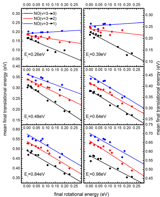
Fig. 19 T - R correlations and anticorrelations in NO scattering from Au(111). \langle E_f \rangle vs. E_{\text{rot}} for NO ( 3 \rightarrow 3, 2, 1 )/Au(111) at various translational energies of incidence. For all cases, the so called “ T - R anticorrelation” is observed manifested in \left| \frac{\partial \langle E_f \rangle}{\partial E_{\text{rot}}} \right| < 1 . The deviations from unity are more pronounced for vibrationally inelastic channels, especially at low values of incident translational energy. From ref. 61 with permission from the PCCP Owner Societies Copyright (2014).
