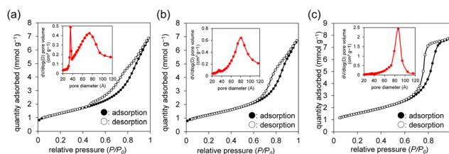
Fig. 6 Nitrogen adsorption-desorption isotherms and BJH pore size distributions (inset) for (a) β-MnO 2 -1, (b) β-MnO 2 -2, and (c) β-MnO 2 -3. (Reproduced from ref. 43 with permission from The American Chemical Society).
