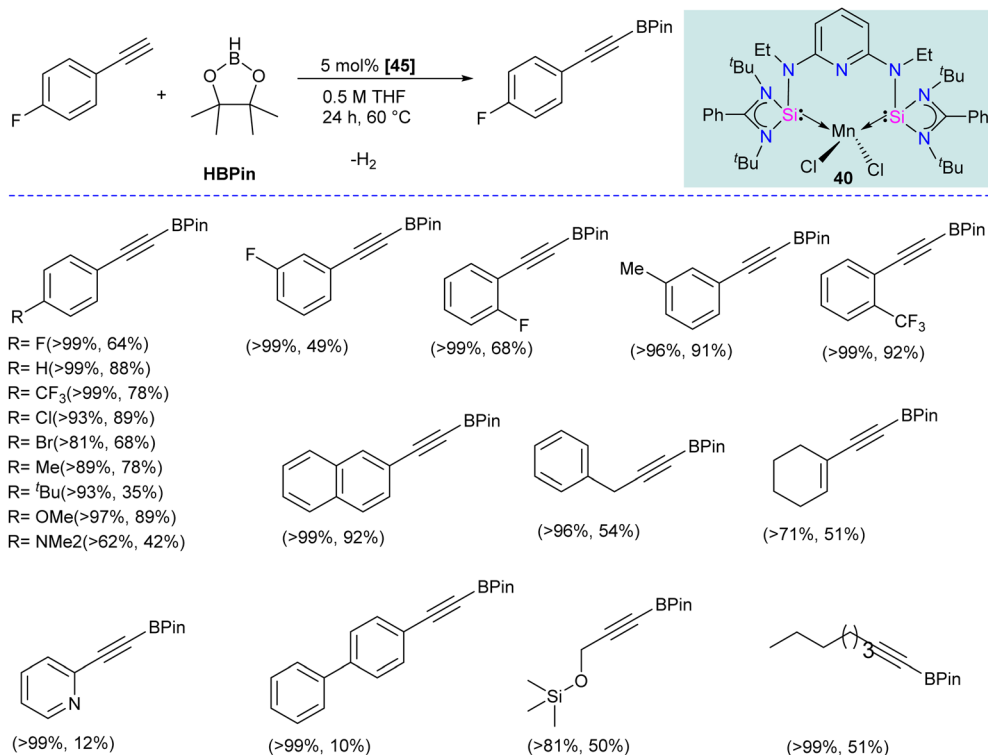
Scheme 17 The catalytic utility of SiNi-MnCl_2 complex 40 in C(sp)-H borylation reactions.
